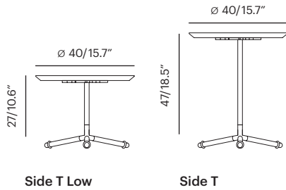
Side T Low
